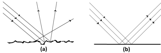
Figure 1. (a) A rough surface reflects light diffusely (b) A plane surface produces specular reflection.
