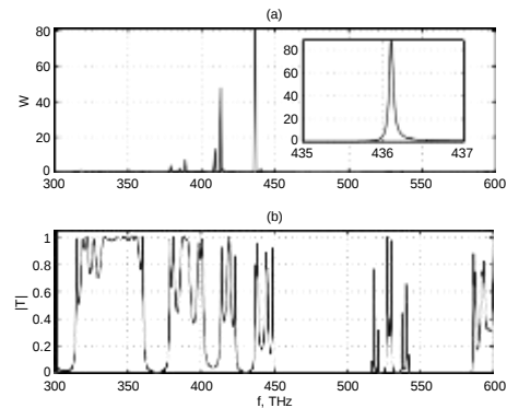
Fig. 4. (a) imaginary parts of tangential component of the Green's function W=G_{\phi\phi}(r, r) for r=900\text{nm} ; (b) Frequency spectrum of transmittance coefficient T for spherical quantum number m=9 . Microsphere is coated by quasiperiodic stack with N=68 (34 of 2-layers blocks, order Fibonacci F_9 ) for \gamma=0.618 . See details in text.
