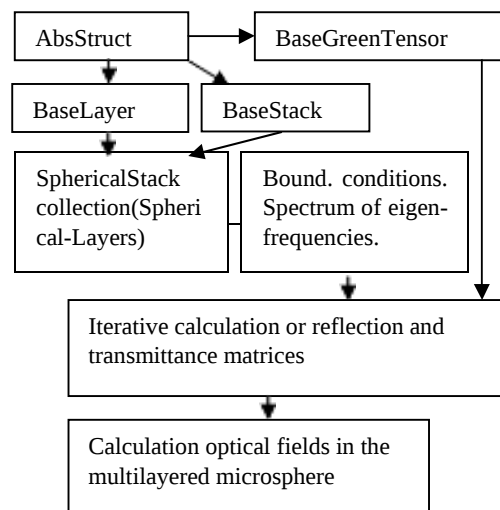
Fig. 2. The hierarchy of main classes in the program code.
