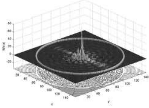
Fig. 6. Spatial structure W(r, \phi) = \text{Im}(G_{\phi\phi}(r, a, \phi)) in a cross-section 0 < r < 21 \mu\text{m} and 0 < \phi < 2\pi of the microsphere with quasiperiodic stack for eigenfrequency f = 436.09 \text{ THz} . A nanoemitter is placed at point a = 900 \text{ nm} . Other parameters are as in Figure 2. One can see the confinement of field in the stack. Outer cycle indicates the external boundary R_{\text{ext}} = 13.8 \mu\text{m} of the quasiperiodic spherical stack.
