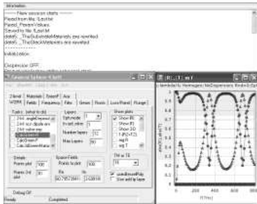
Fig. 3. Graphical user interface and example calculation of the reflection and transmittance coefficients.
