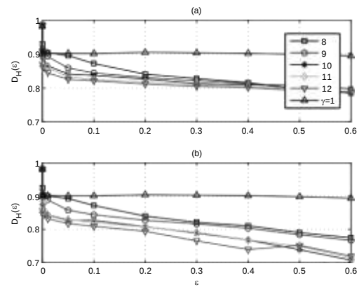
Fig. 7. Fractal (capacity) dimension D_H(\epsilon) for Fibonacci stack F_j with j=8\div 12 and \gamma=0.5 . The last curve shows the periodic stack case with F_{\infty} and \gamma=1 . (a) lossless stack; (b) dissipative stack.
